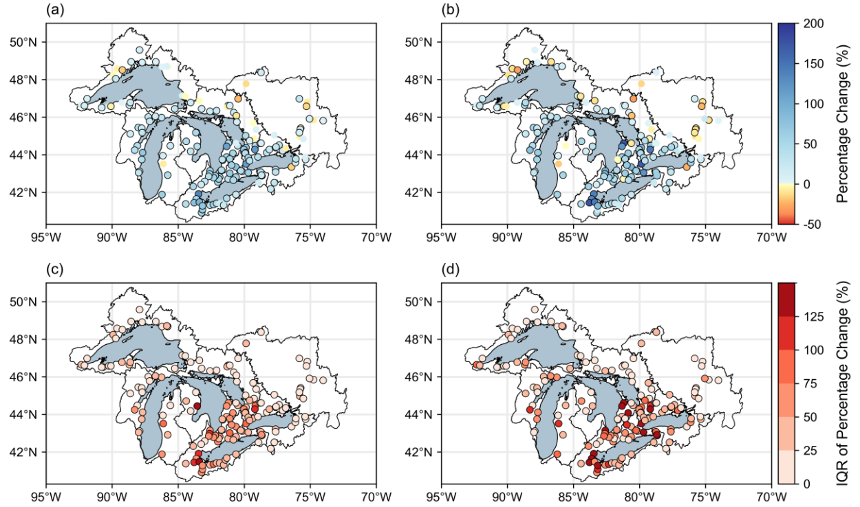
Figure 2: Spatial distribution of projected changes in flood magnitude across the Great Lakes basin. Panels (a) and (b) show the multi-model ensemble median (from 8 GCMs) of the percentage change in flood magnitude between the historical period (1985–2014) and the future period (2071–2100) for the (a) 5-year and (b) 100-year return periods, respectively. Dots outlined in black indicate gauges where the projected change meets the model agreement threshold ( \geq 67\% of GCMs). Panels (c) and (d) show the corresponding IQR of percentage change across the 8 GCMs for the (c) 5-year and (d) 100-year return periods.
