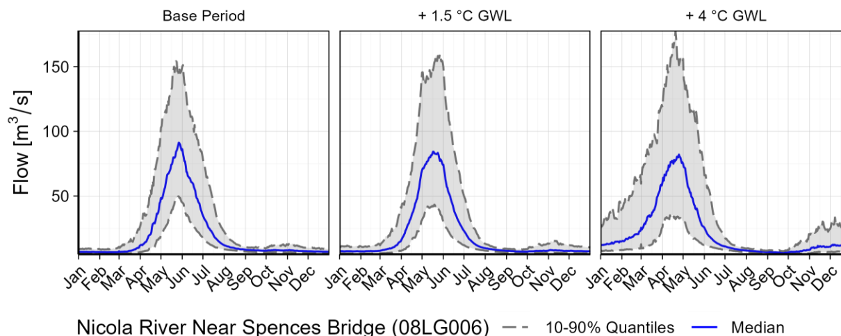
Figure 5: Projected daily hydrographs under warming scenarios at the Nicola River near Spencer Bridge hydrometric station based on daily simulations of the Variable Infiltration Capacity hydrologic model. For each day of the year, the multi-model ensemble's median and 80% confidence interval are presented.
