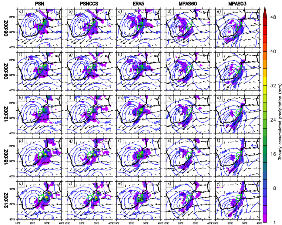
Figure 1: 500 hPa geopotential Height (blue contour; m), 850 hPa wind field (black vector; \text{ms}^{-1} ) and the COL-associated 3-hourly accumulated precipitation (shaded, mm) as represented by the observation (PSN, PSNCCS), ERA5 reanalysis and MPAS simulations (MPAS60 and MPAS03). The green polygon represents the KwaZulu-Natal province of South Africa.
