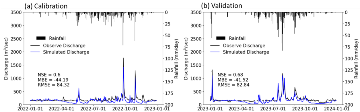
Figure 5: Comparison between observed discharge and simulated discharge at the SanIsidro gauging station: (a) model calibration for 2022 and (b) model validation for 2023
