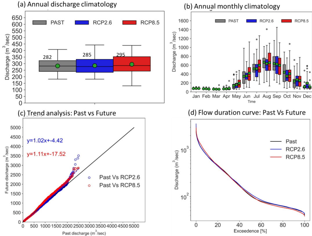
Figure 7: Comparison of basin-averaged discharge climatology and extremes at San-Isidro gauging station between historical and RCP scenario; (a) annual discharge climatology, (b) annual monthly climatology, (c) trend analysis of daily discharges, and (d) flow duration curve. The green circle in the box-whisker plot represents the mean values.
