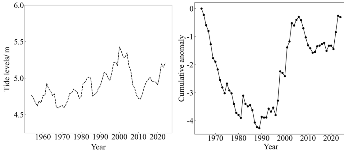
Figure 2: The 5-year sliding average curve and cumulative anomaly of H_{max} at Wusong stations.
