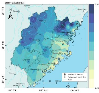
(a) Daily average rainfall
