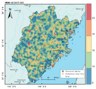
(g) Small watershed area
