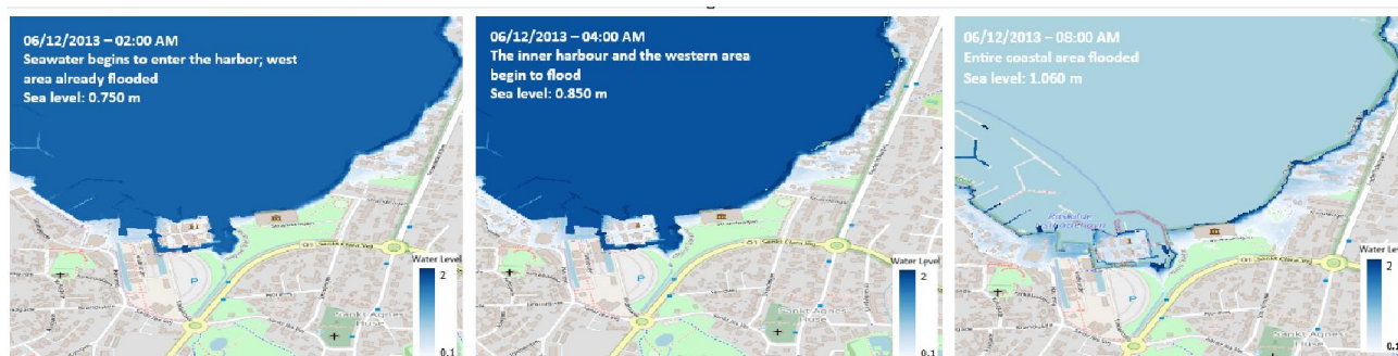
Figure 3. Simulated temporal evolution of flooding in the Roskilde Harbour area during the Bodil storm. Snapshots at 02:00, 04:00, and 08:00 on 6 December 2013.
